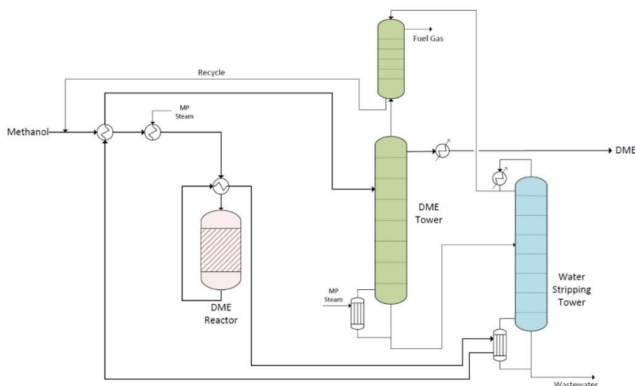
DME Process Diagram
